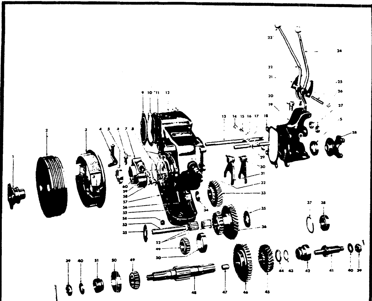
TRANSFER CASE EXPLODED VIEW (FOR MODELS CJ2A &amp; 3A)
