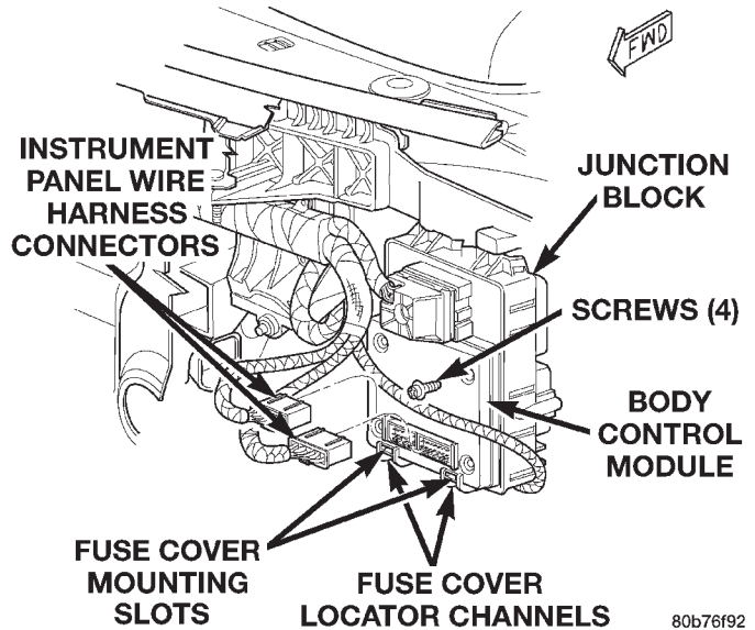
Fig. 3 Instrument Panel Fuse Cover Locator Channels
