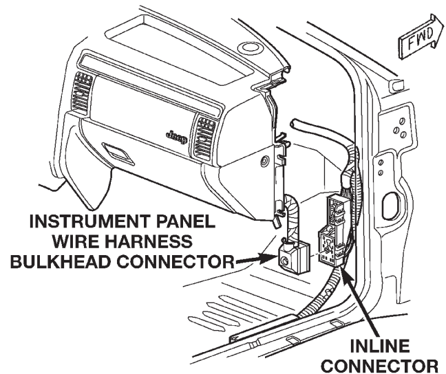
Fig. 41 Instrument Panel to Driver Side Cowl Side Inner Panel Mounting
