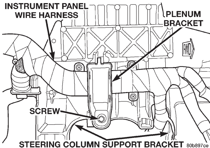
Fig. 48 Instrument Panel Plenum Bracket Remove/Install
