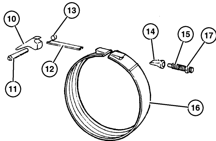
REVERSE BAND
