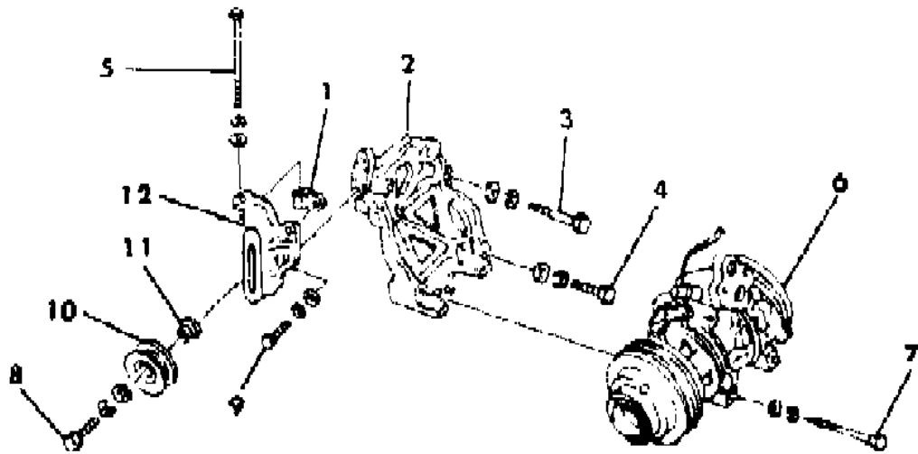
2.0 LITER ENGINE
