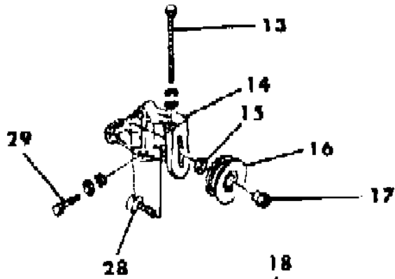
2.0 LITER ENGINE
