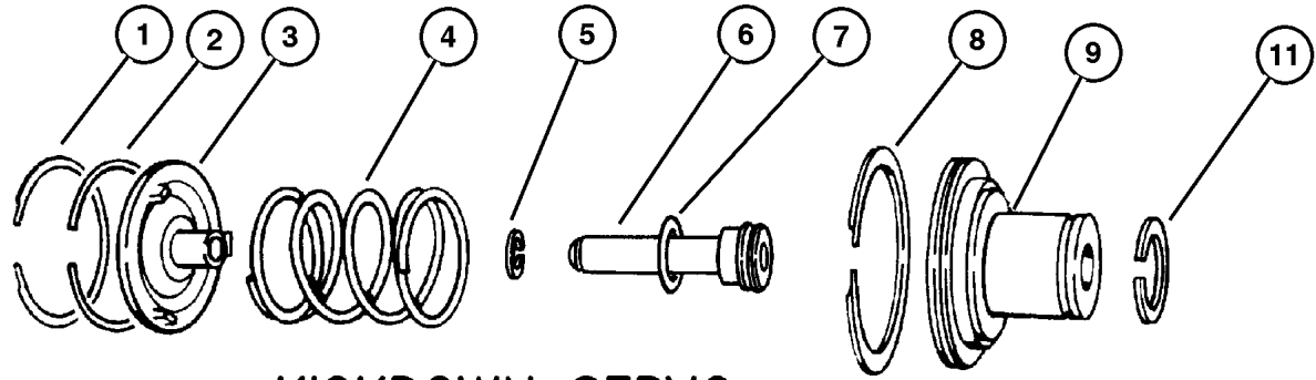
KICKDOWN SERVO
