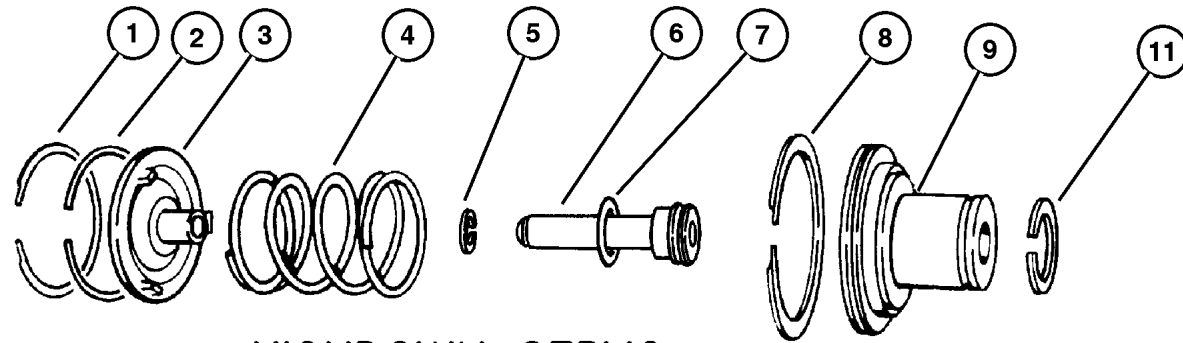
KICKDOWN SERVO
