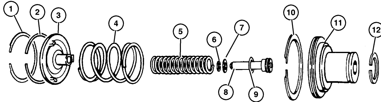
KICKDOWN SERVO
