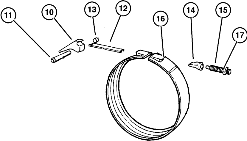
REVERSE BAND
