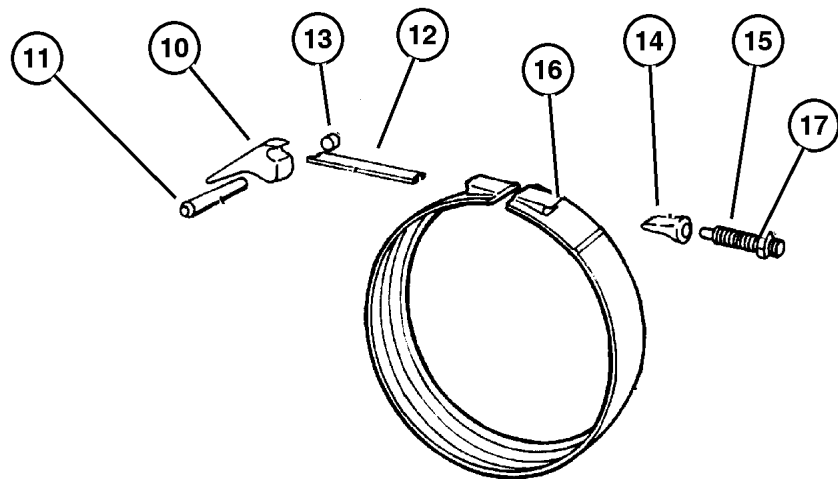
REVERSE BAND
