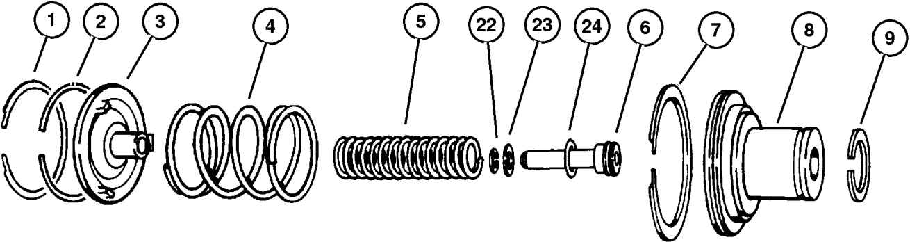
KICKDOWN SERVO
