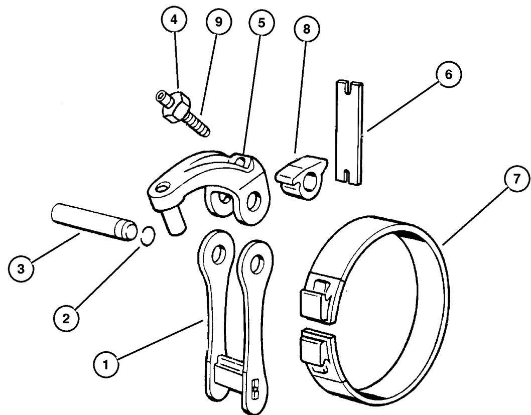
REVERSE BAND
