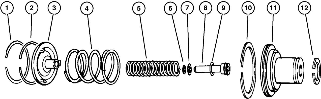
KICKDOWN SERVO
