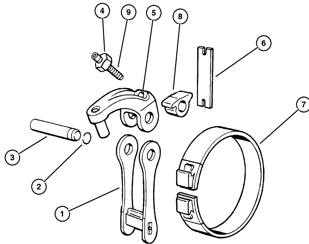
REVERSE BAND
